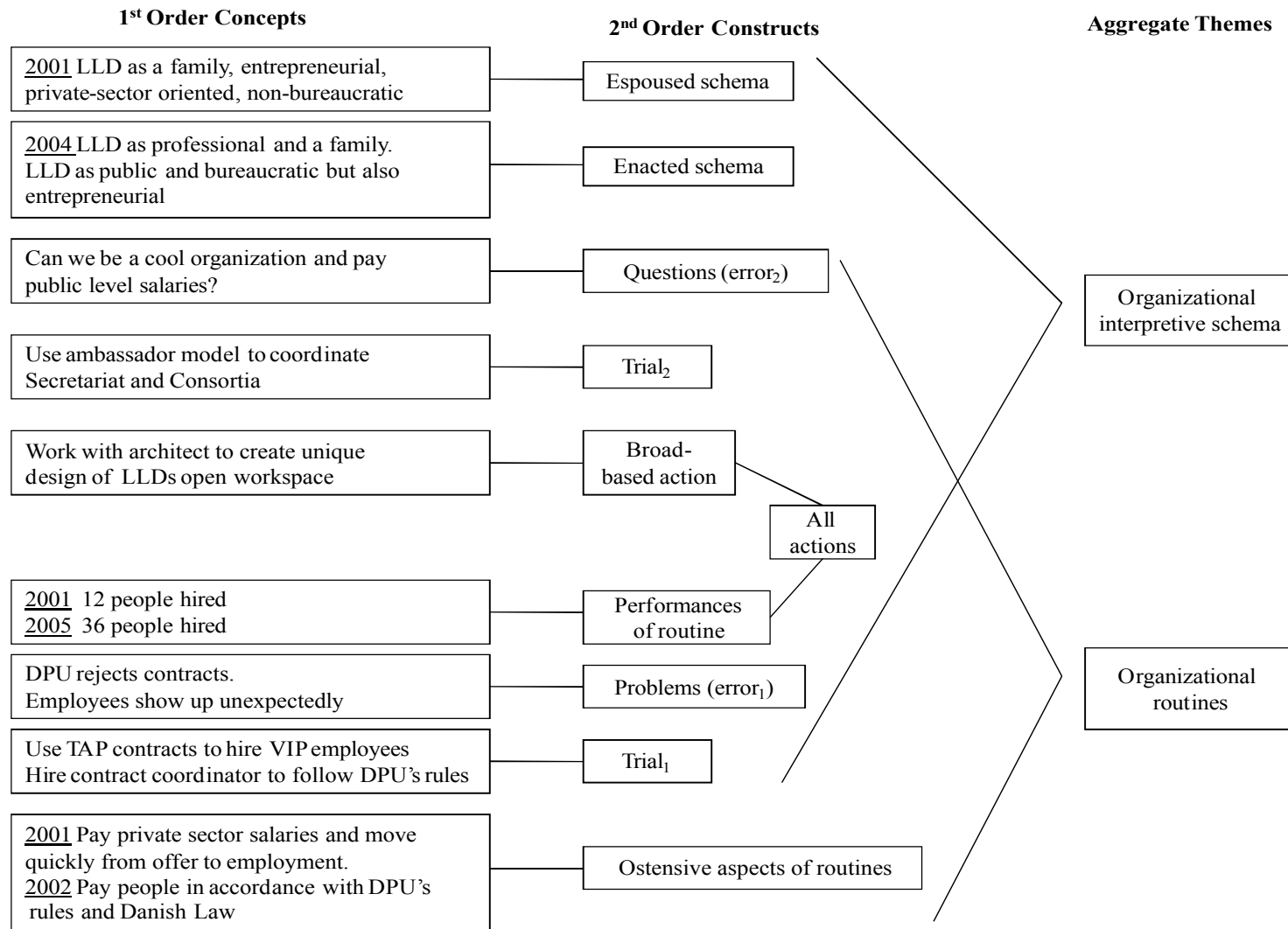
FIGURE 1 Data Structure
